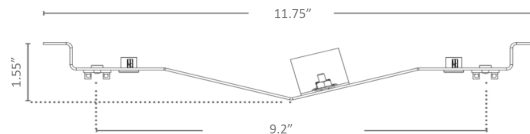
2 x 2 and 2 x 4 Troffer Retrofit
